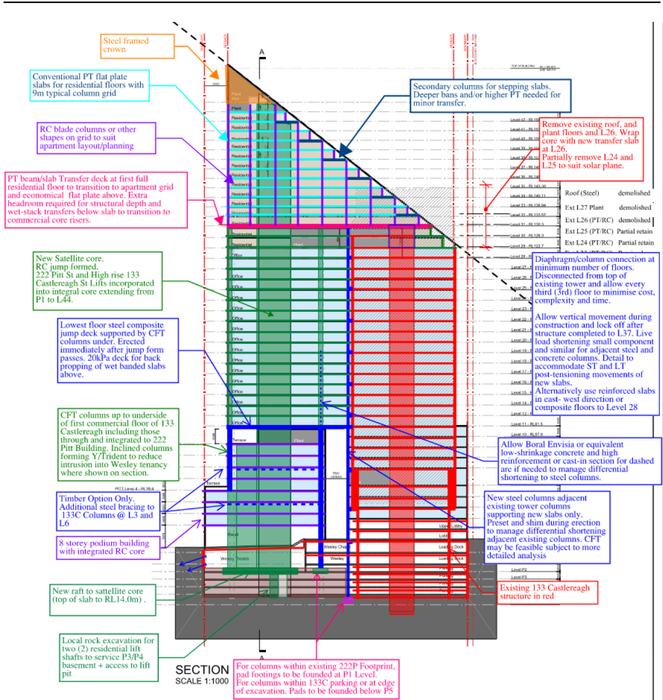
Figure 1: East-west structural section in the mixed-use scenario
